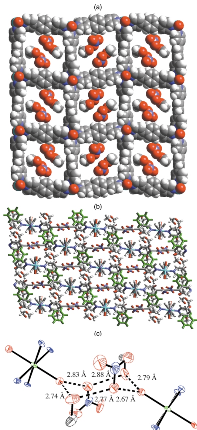
Fig. 1 The crystal structure of complex 4 . (a) Space filling representation of the open square grid network. The square cavities are occupied by two O–H...O dimers of MeOH and nitrate. (b) Offset packing of the grids with an interlayer separation of 4.7 Å. Note the benzene molecules between the grids. (c) An ORTEP 15 drawing (40% probability) showing the chair conformation of synthon I .
